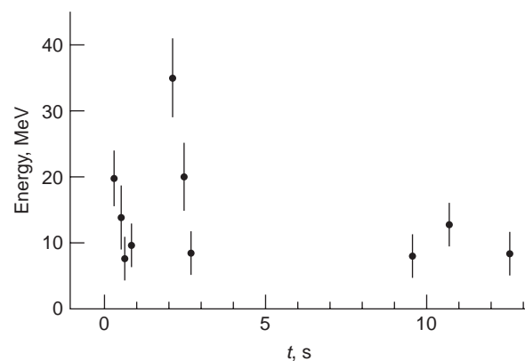
FIGURE 12-33 Electron antineutrino energy versus arrival time in the Kamiokande detector in Japan for antineutrinos emitted by the supernova 1987A. The spread in arrival times (about 13 s) permits a calculation of an upper limit to the mass of the \bar{\nu}_e .
